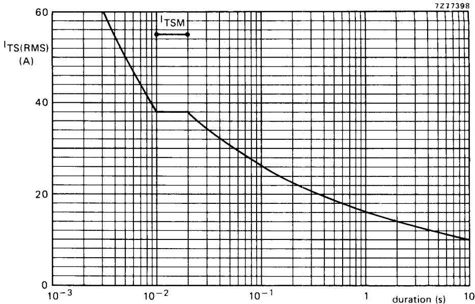
Fig.6 Maximum permissible non-repetitive r.m.s. on-state current based on sinusoidal currents ( f = 50 \text{ Hz} ); T_j = 120 \text{ }^\circ\text{C} prior to surge. The triac may temporarily lose control following the surge.
