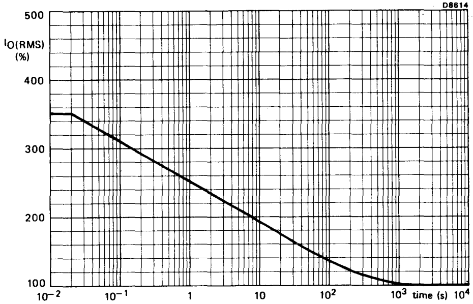
Fig.4 Maximum permissible duration of steady overload (provided that T_{mb} does not exceed 120\text{ }^{\circ}\text{C} during and after overload) expressed as a percentage of the steady state r.m.s. rated current. For high r.m.s. overload currents precautions should be taken so that the temperature of the terminals does not exceed 125\text{ }^{\circ}\text{C} . During these overload conditions the triac may lose control. Therefore the overload should be terminated by a separate protection device.
