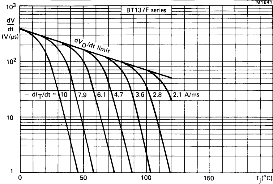
Fig.10 Typical commutation dV/dt for BT137F series versus T_j . The triac should commute when the dV/dt is below the value on the appropriate curve for pre-commutation di_T/dt .
