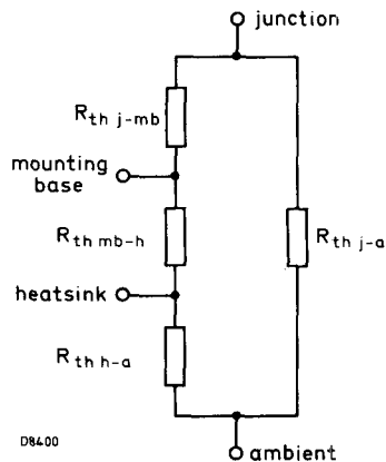
Fig.2 Components of thermal resistance.
