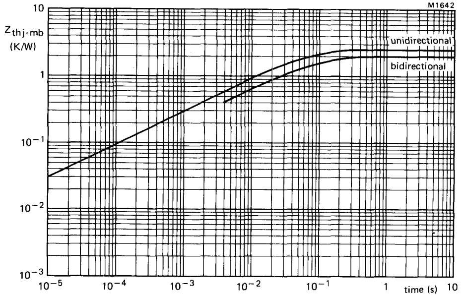
Fig.5 Thermal impedance as a function of dissipation time.
