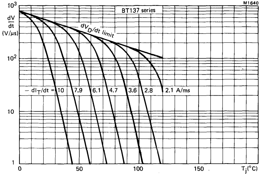
Fig.8 Typical commutation dV/dt for BT137 series versus T_j . The triac should commute when the dV/dt is below the value on the appropriate curve for pre-commutation di_T/dt .
