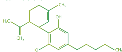
Cannabidiol
