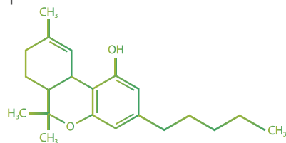
Tetrahydrocannabinol
